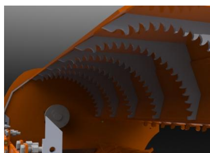
Detaliu fierastrai interior
